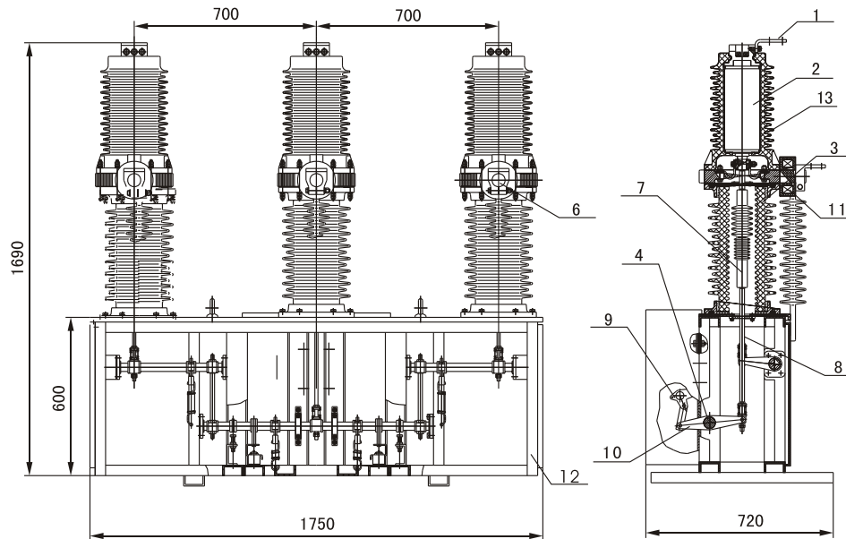
ZW37(G)-40.5 Outline dimension and installation drawing
